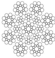
Multilift DPS Steel wire rope Multilift double parallel seal
